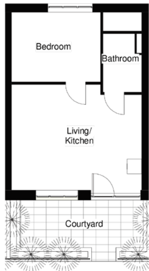
Flat Type 2 Flat No. 22, 23, 24
