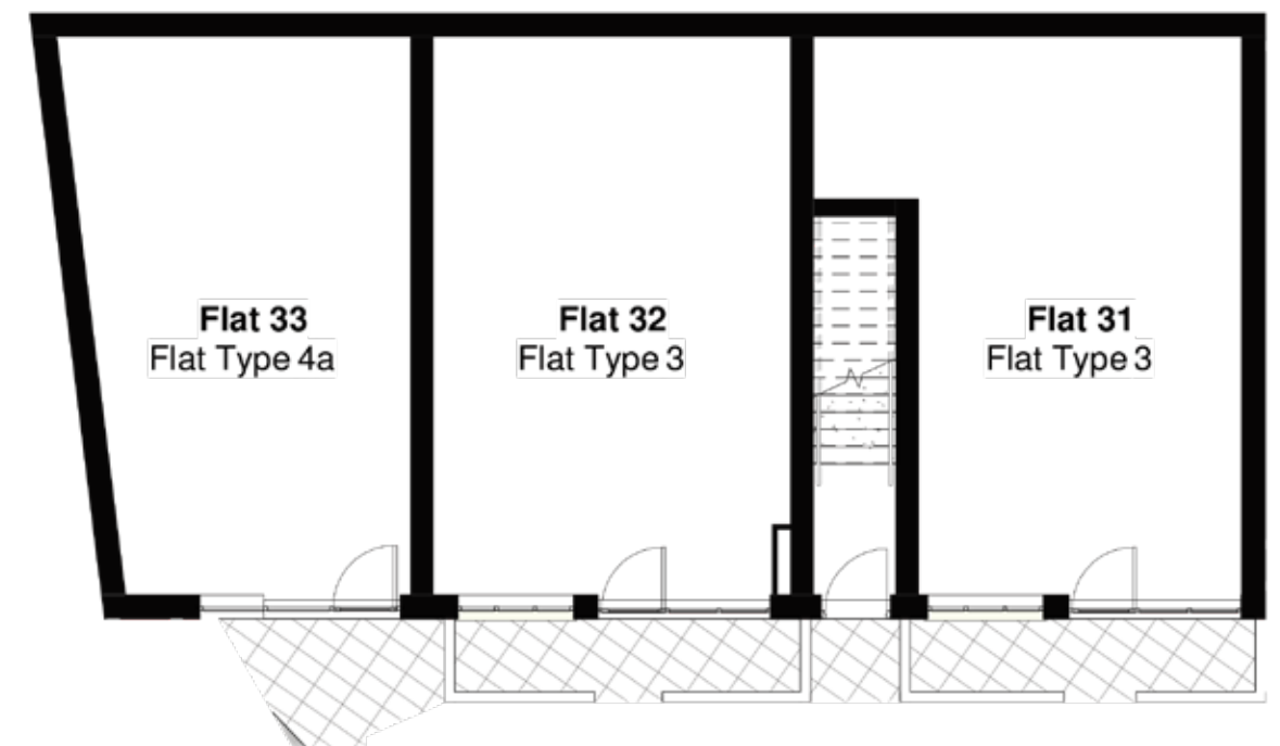
Block C Ground Floor
