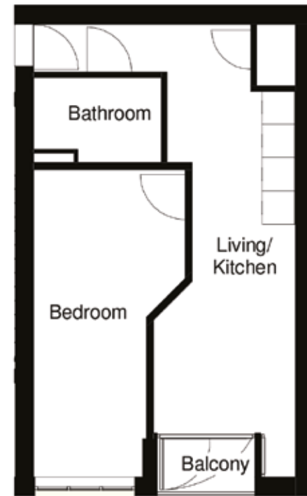
Flat Type 8 Flat No. 34, 35
