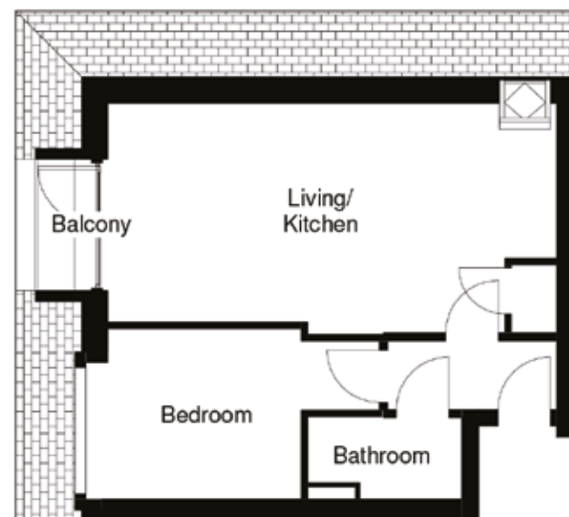
Flat Type 9 Flat No. 14, 15, 16, 17, 18
